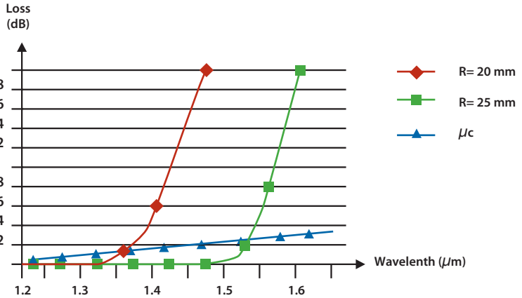
The effects of macro bending on a fiber
