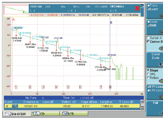
Automatic event detection using the JDSU T-BERD/MTS platforms
