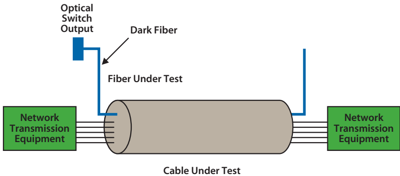
Out-of-service monitoring of a link
