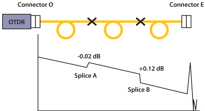
OTDR measurement from connector O to connector E (O -> E)
