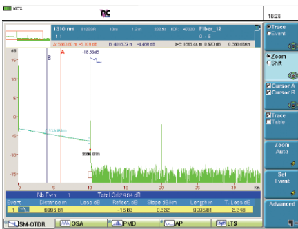
An example of a ghost in the signal noise
