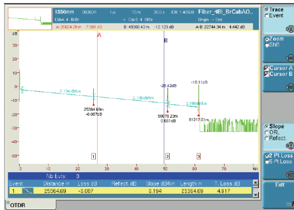
Manual measurement using cursors A and B
