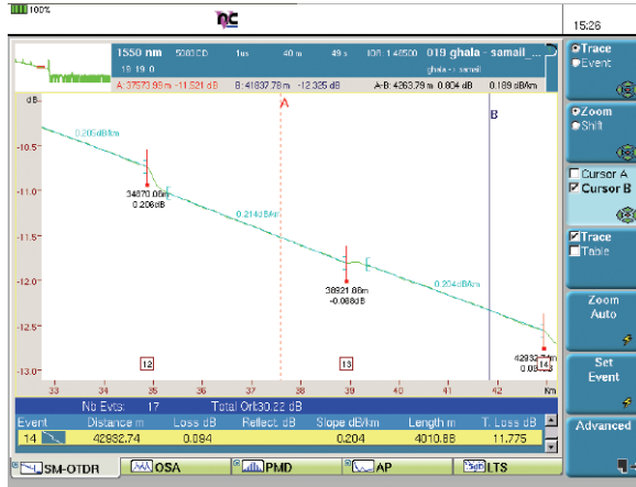
A splice gain on an OTDR trace
