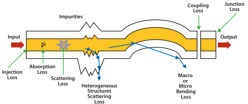
Link loss mechanisms
